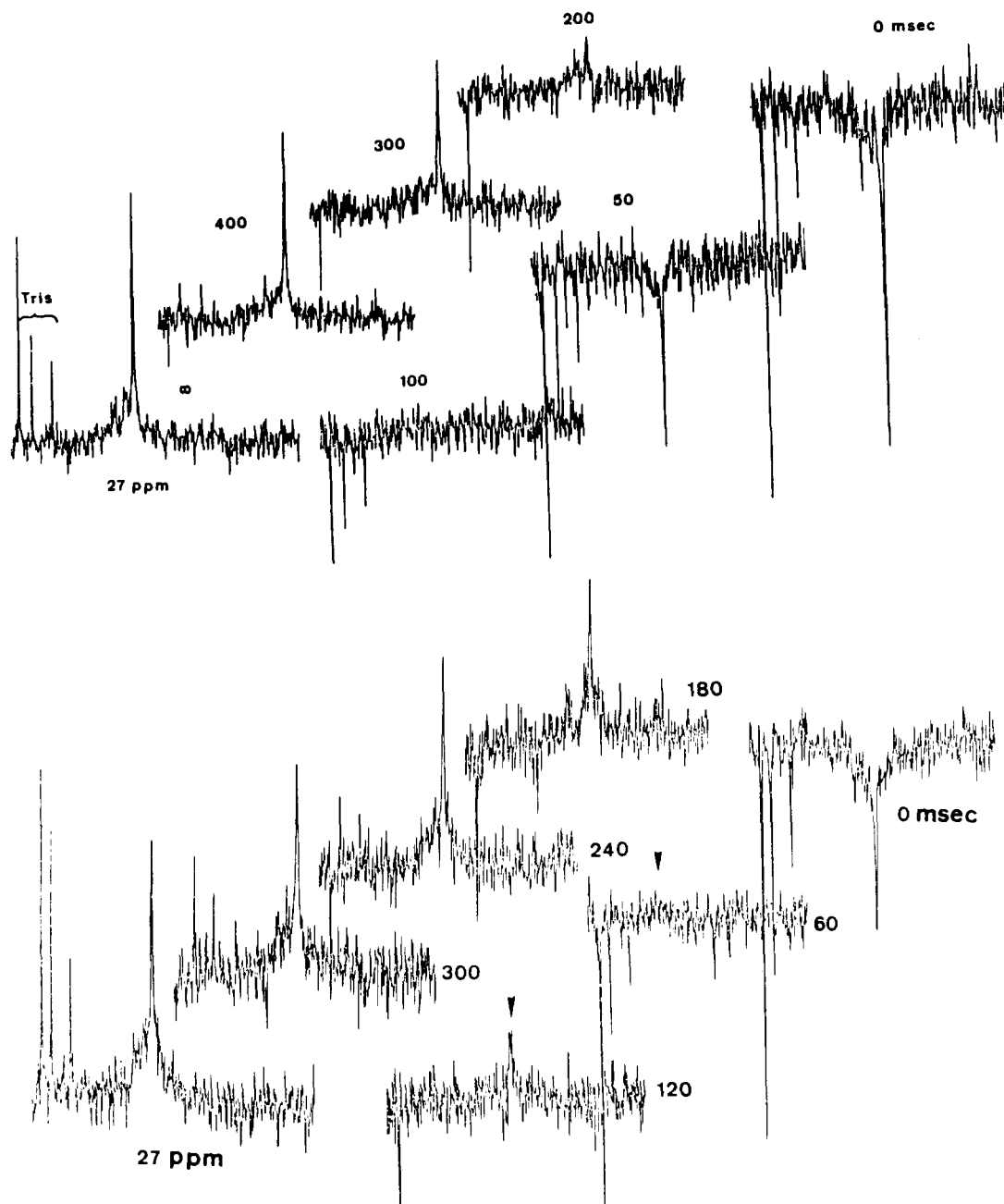
FIGURE 5: Measurement of the spin-lattice relaxation time ( T_1 ) of [11\text{-}^{13}\text{C}] dioleoyllecithin as phospholipid vesicles alone or complexed with D- \beta -hydroxybutyrate apodehydrogenase. Samples were prepared and partially relaxed ^{13}\text{C} NMR spectra obtained as described in Figure 3 except that [11\text{-}^{13}\text{C}] dioleoyllecithin was used in place of soybean [N\text{-}^{13}\text{CH}_3] lecithin. The resonance of 11\text{-}^{13}\text{C} of [11\text{-}^{13}\text{C}] dioleoyllecithin is at 27 ppm relative to tetramethylsilane. (A) Partially relaxed spectra of 10 mg of [11\text{-}^{13}\text{C}] dioleoyllecithin as codispersion with mitochondrial phosphatidylethanolamine (PE) and diphosphatidylglycerol (DPG) (PC/PE/DPG phosphorus ratio of 1.0:0.8:0.2) at 20 °C in \sim 3 mL of NMR assay buffer (cf. Figure 3). Number of scans = 6000. T_1 , computed from the slope of \ln(M_0 - M_z) vs. t (cf. Figure 3), was 211 \pm 12 ms. (B) Partially relaxed spectra of 10 mg of [11\text{-}^{13}\text{C}] dioleoyllecithin as codispersion (cf. Figure 5A) complexed with 12 mg of D- \beta -hydroxybutyrate apodehydrogenase (BDH) in the presence of 0.5 mM NADH in \sim 3 mL of NMR assay buffer at 6 °C. Number of scans = 10000. T_1 was calculated to be 105 \pm 25 ms. It should be noted that the base of the resonance line of the 11\text{-}^{13}\text{C} of the dioleoyllecithin is broadened after complex formation with the apodehydrogenase. The peak heights of the spike and the broad base were found to be proportional at the different delay times so that the T_1 times for both components of the resonance are similar. In the limit, the sample with the most D- \beta -hydroxybutyrate apodehydrogenase (4.8 mg of BDH per mg of lecithin) has lost the sharp spike in the 27-ppm resonance, and only the broad base of the resonance can be observed (not shown).
